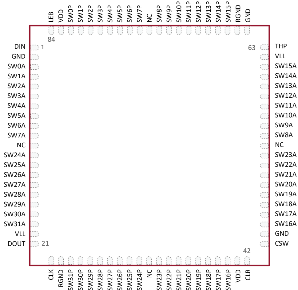
TOP VIEW
