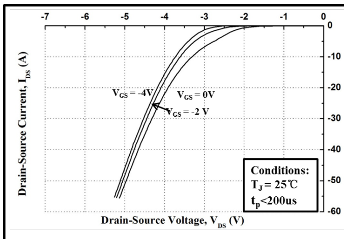
Figure 8. Body Diode Characteristic at 25°C
