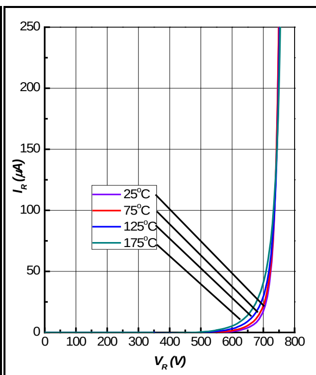
Figure 2. Reverse Characteristics
