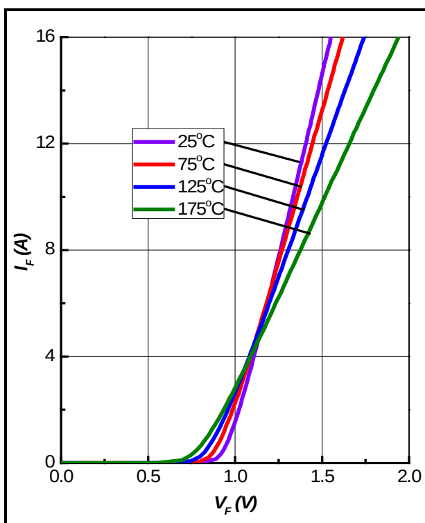
Figure 1. Forward Characteristics
