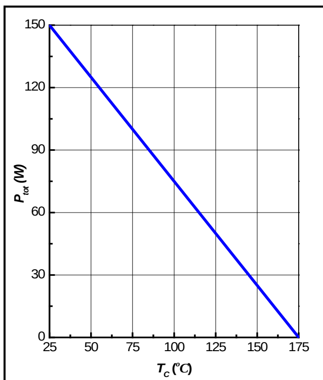
Figure 3. Power Derating
