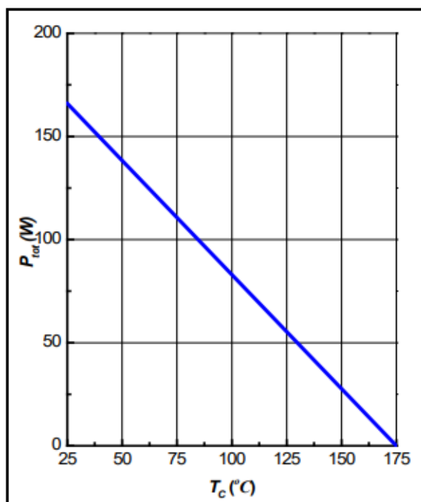
Figure 3. Power Derating
