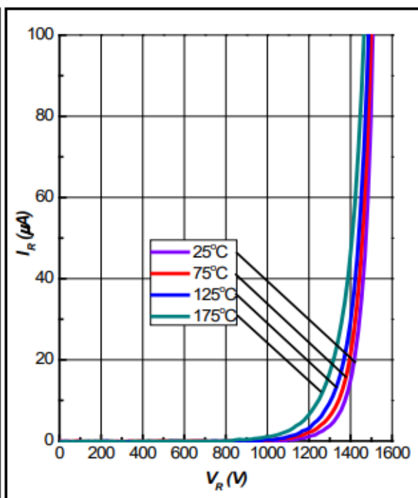
Figure 2. Reverse Characteristics
