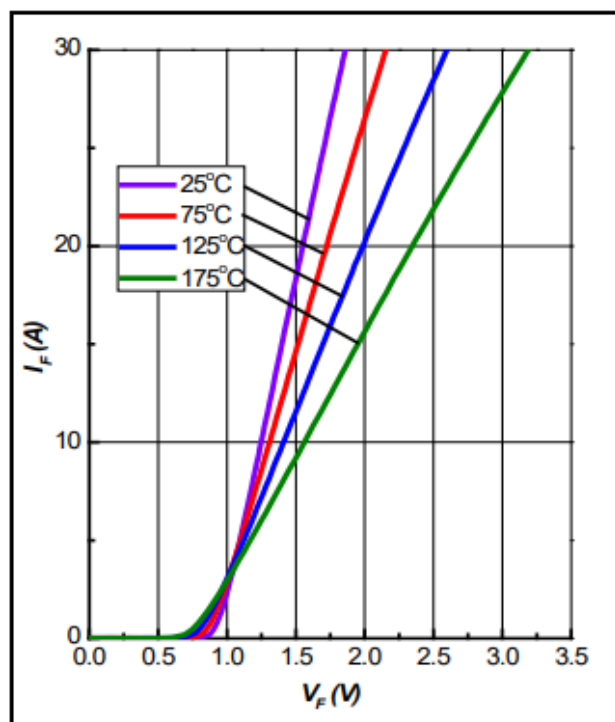
Figure 1. Forward Characteristics
